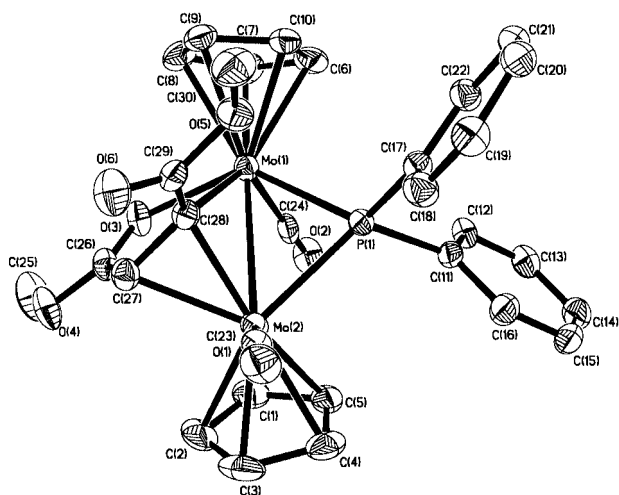
Fig. 1 Molecular structure of complex 3 in the crystal, showing the numbering scheme.
